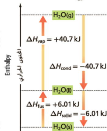
Phase Changes for Water
