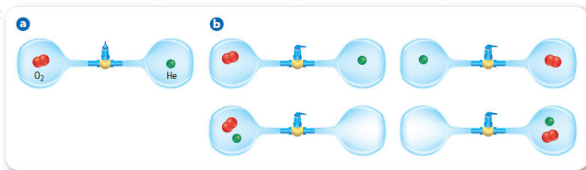
■ Figure 18 In a , an oxygen molecule and a helium atom are each confined to a single bulb. When the stopcock is opened in b , the gas particles move freely into the double volume available. Four arrangements of the particles, which represent an increase in entropy, are possible at any given time.
