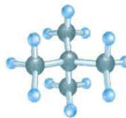
2,2-Dimethylpropane bp = 9^\circ C
