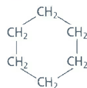
Condensed structural formula
