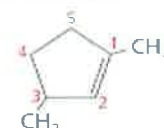
b. Cyclic alkenes
