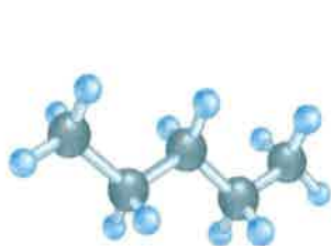
Pentane bp = 36^\circ C
